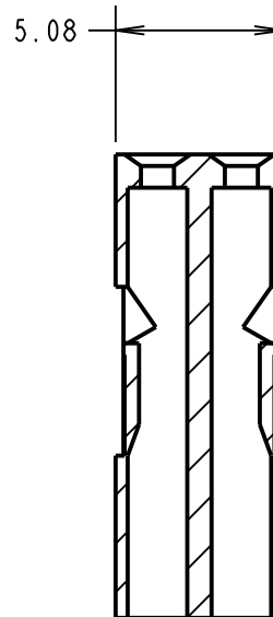
SECTION X-X
