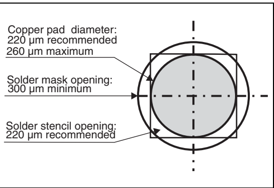
Figure 18. Footprint
