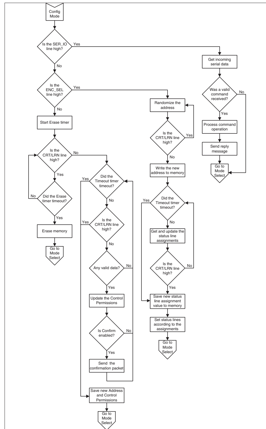
Figure 26: MT Series Transcoder Configure Flowchart
