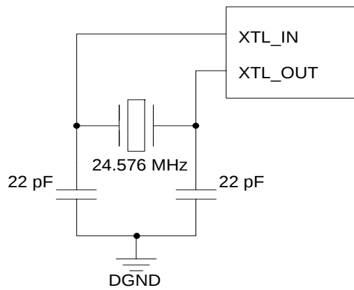
Figure 24. External Crystal
