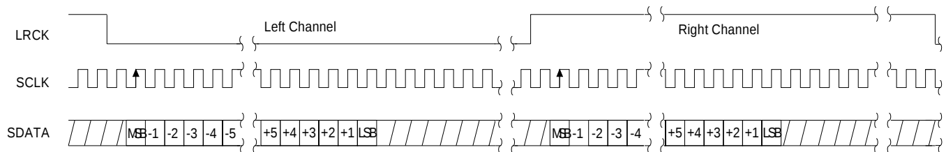
Figure 17. Serial Data Format 0 (I²S)
