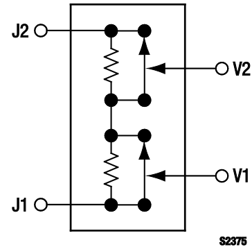
Figure 1. SKY12324-73LF Block Diagram
