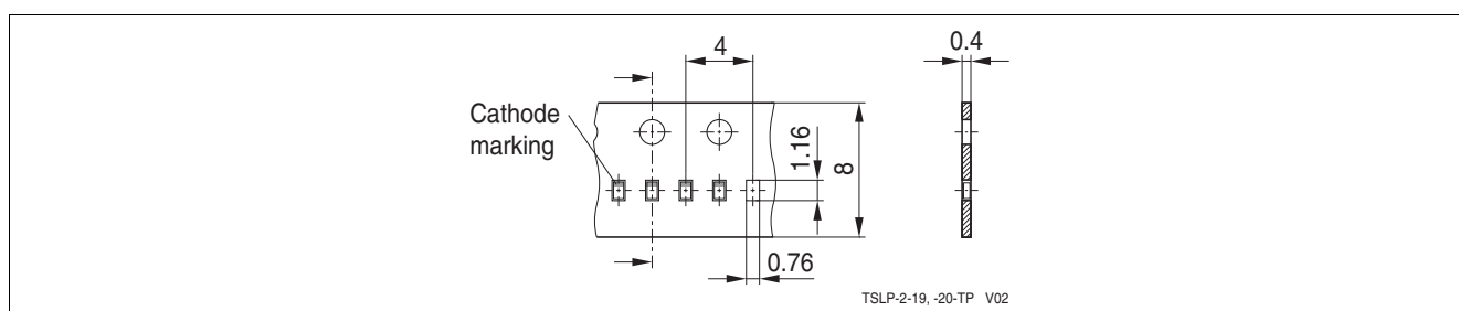
Figure 4-7 TSLP-2-20: Packing
