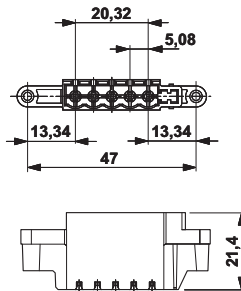
Dimensioned drawing
