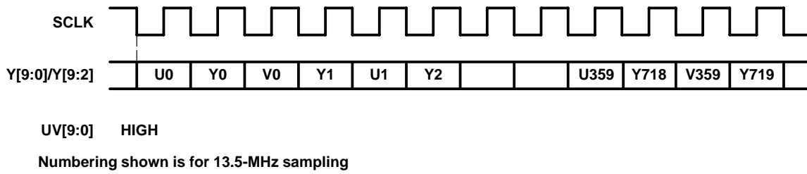
Figure 2–26. 10-/8-Bit 4:2:2 Output Format
