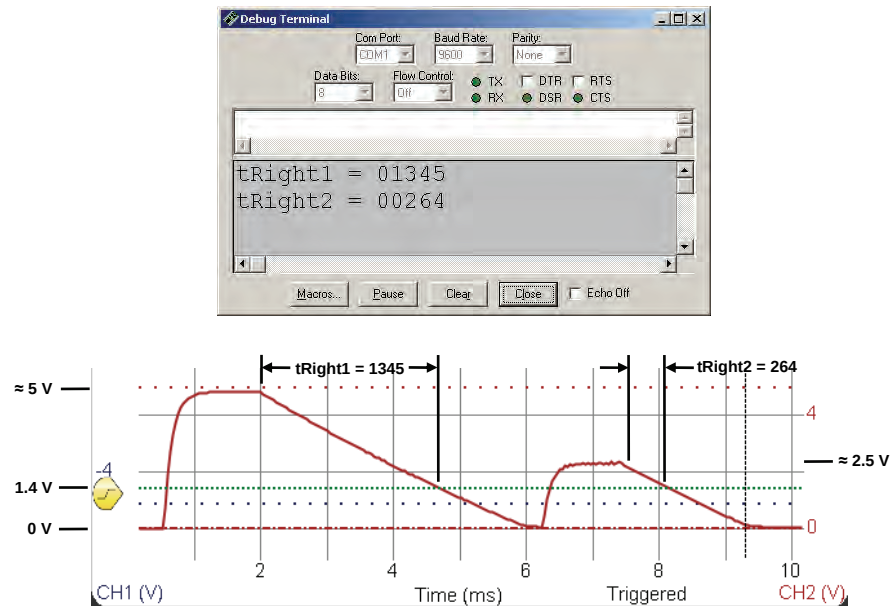
Figure 6-14: Debug Terminal and Oscilloscope Views of HighVsPwmInRctime.bs2
