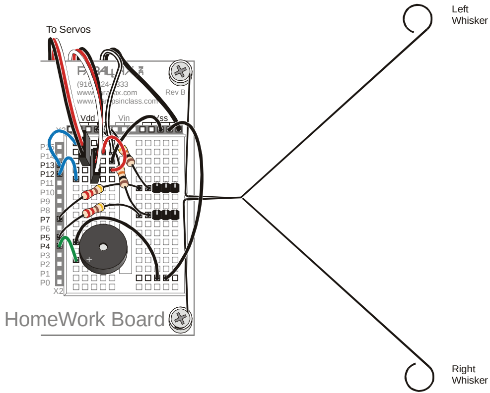
Figure 5-6: Whisker Wiring Diagram for the HomeWork Board
