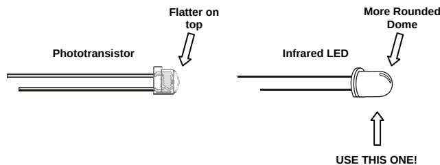
Figure 7-5 Distinguishing Phototransistors from Infrared LEDs
