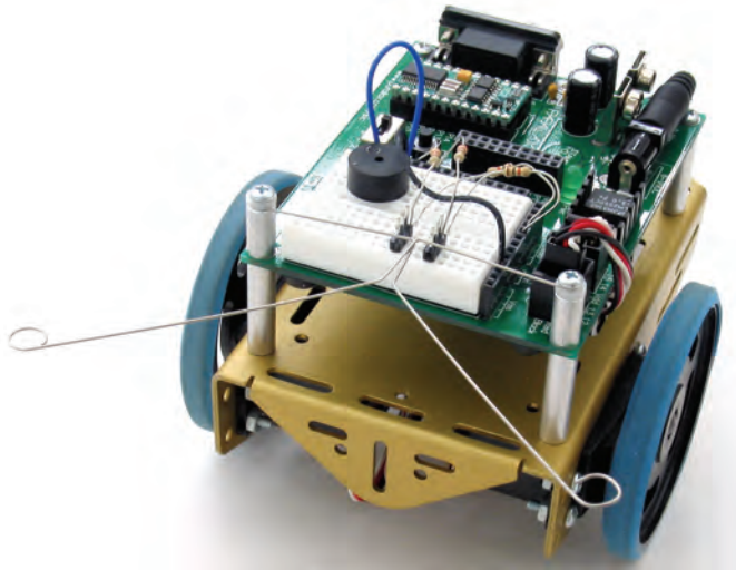
Figure 5-1 Boe-Bot with Whiskers
