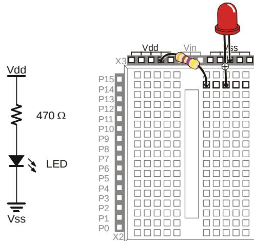
Figure B-4 Example Schematic and Wiring Diagram
