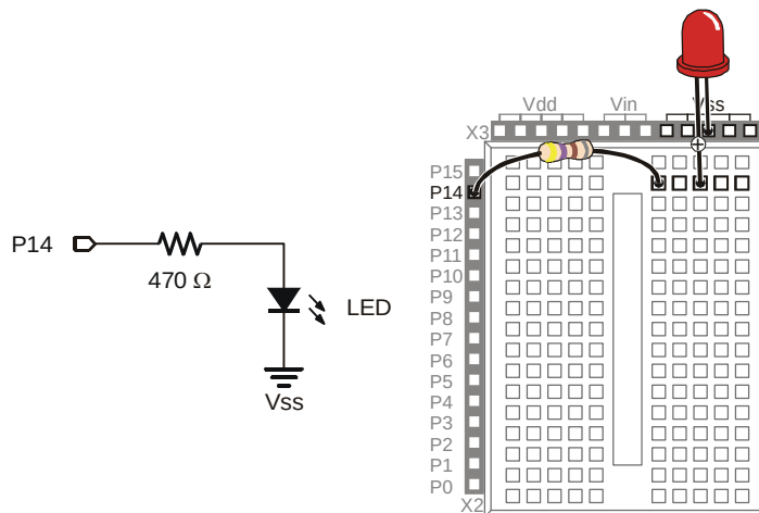
Figure B-5 Example Schematic and Wiring Diagram
