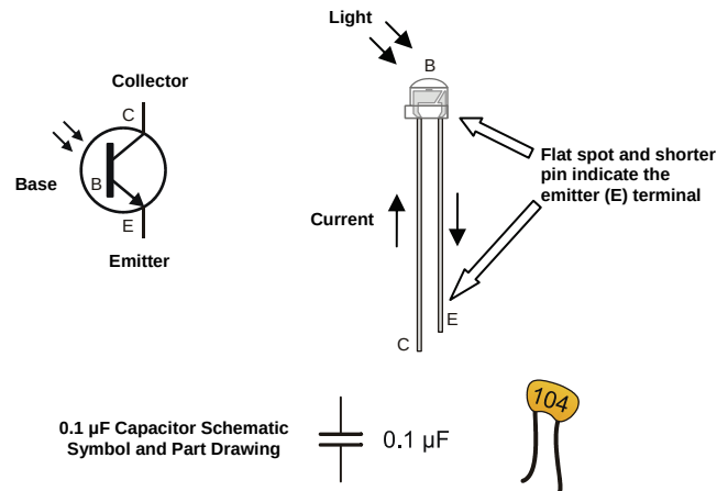
Figure B-6 Part Drawings and Schematic Symbols Phototransistor (top) Non-polar capacitor (bottom)
