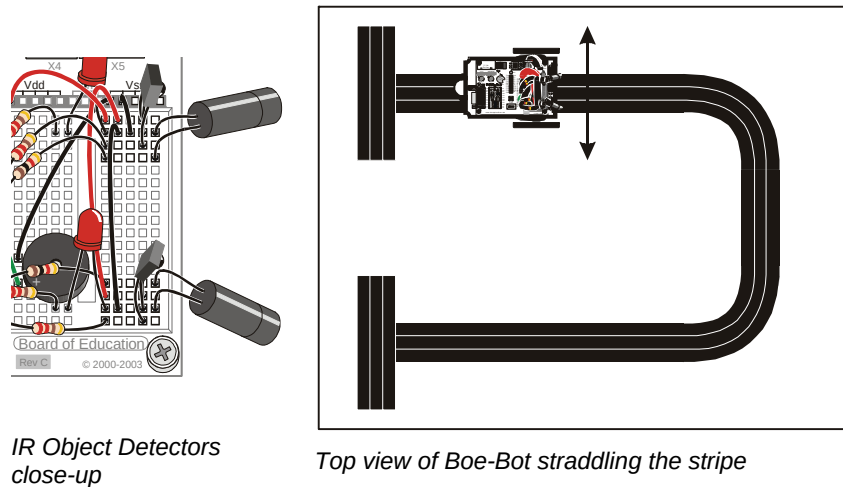
Figure 8-12: Stripe Scan Test
