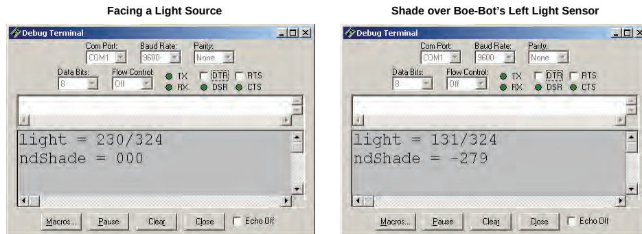
Figure 6-16: Example Shadow Tests with LightSeekingDisplay.bs2
