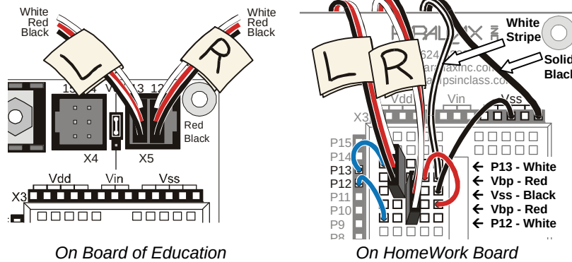
Figure 3-10 Servo Ports Reconnected
