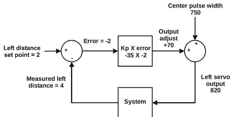
Figure 8-5 Proportional Control Block Diagram for Left Servo and IR Object Detector
