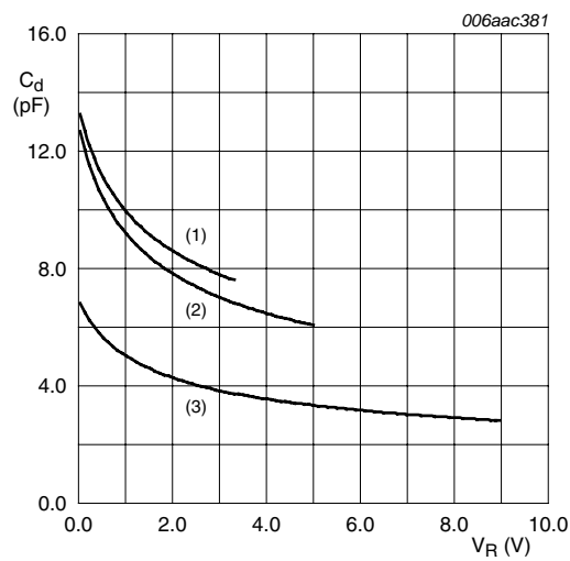
f = 1\text{ MHz}; T_{amb} = 25\text{ }^{\circ}\text{C} (1) PESD3V3V4UK (2) PESD5V0V4UK (3) PESD9V0V4UK
