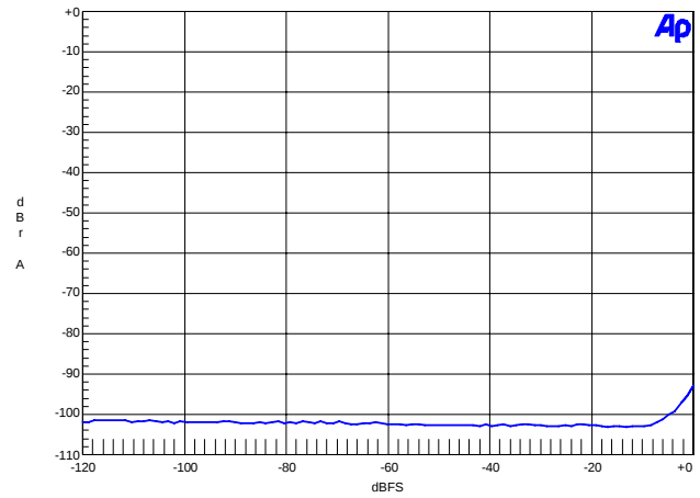
Figure 26. 192 kHz, THD+N vs. Level
