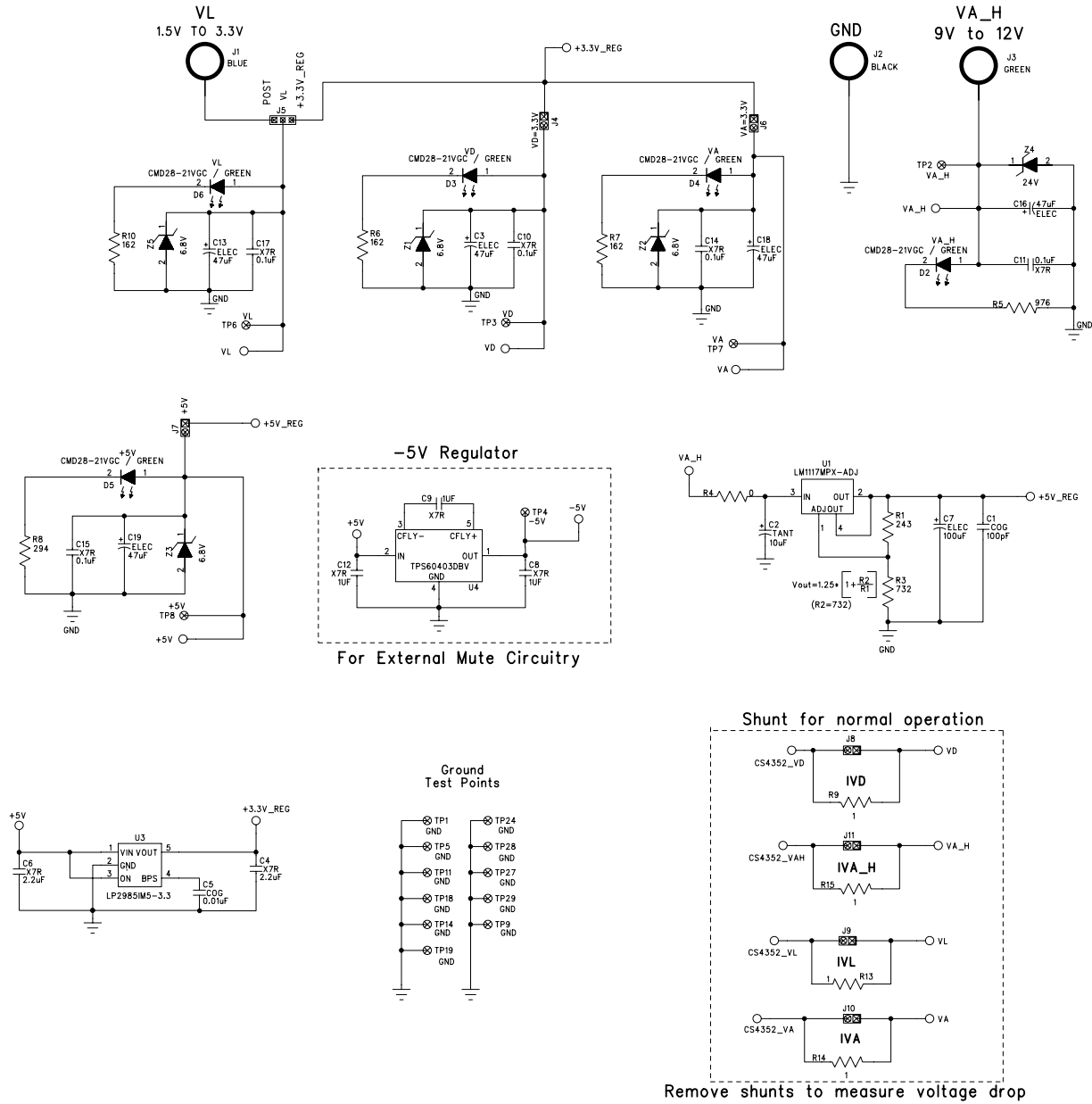
Figure 36. Power
