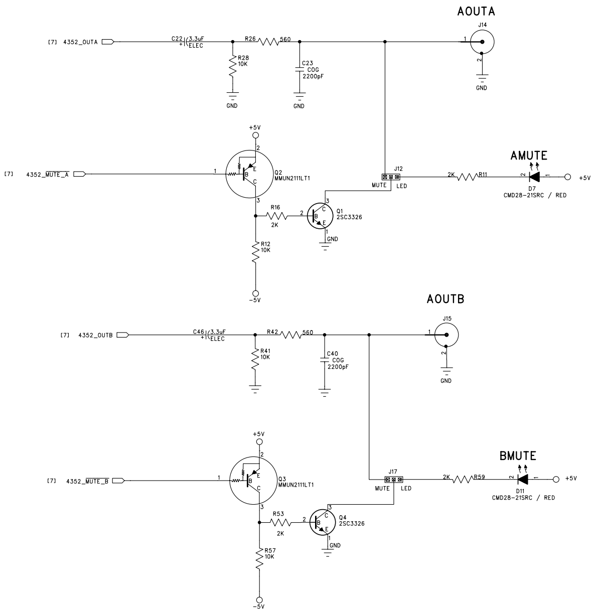
Figure 33. Analog Outputs
