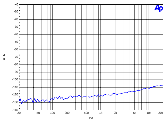
Figure 9. 48 kHz, Crosstalk
