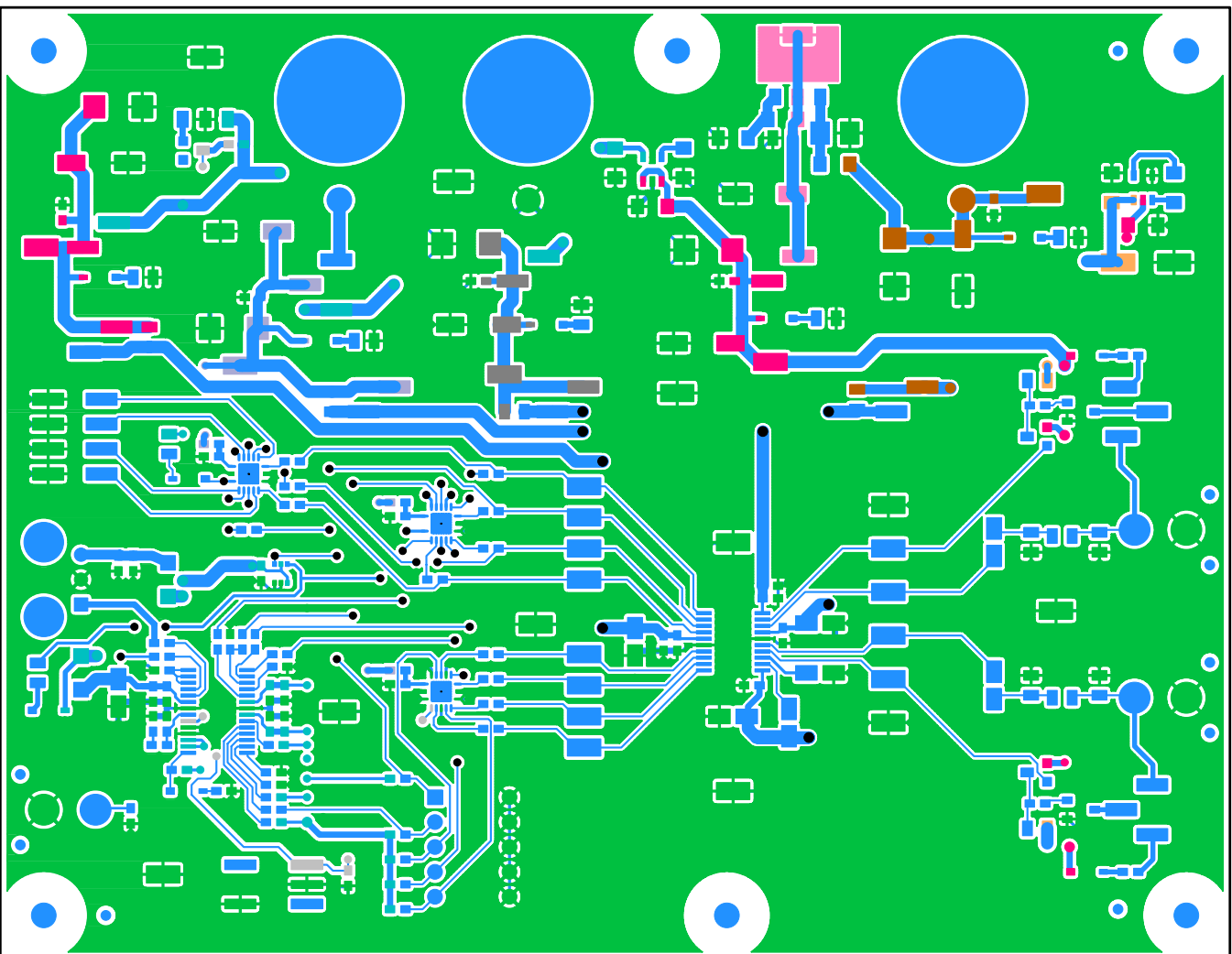
Figure 38. Top Side
