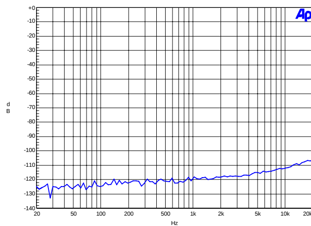
Figure 29. 192 kHz, Crosstalk
