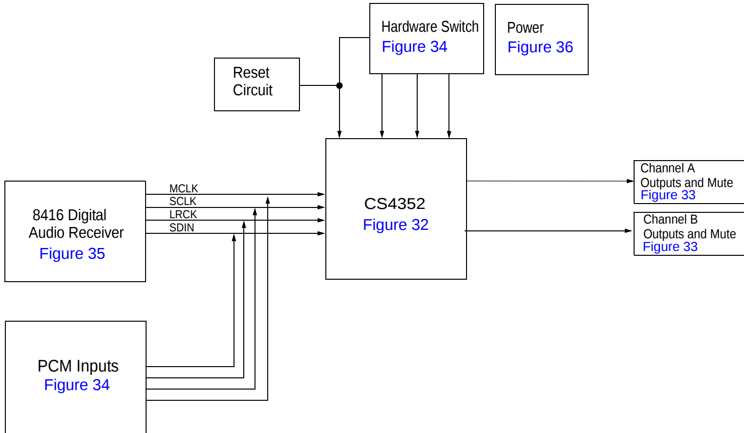
Figure 31. System Block Diagram and Signal Flow
