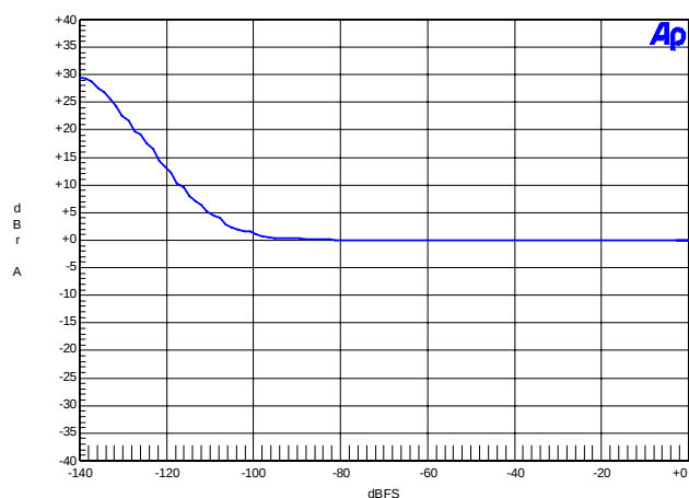
Figure 7. 48 kHz, Fade-to-Noise Linearity
