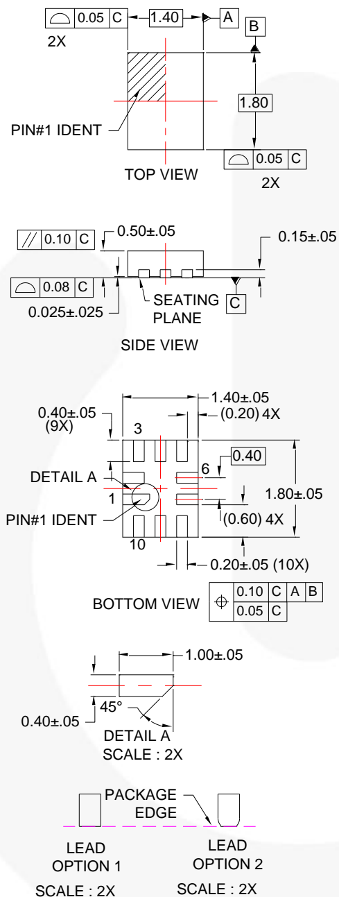
Figure 4. 10-Lead UMLP Package Drawing
