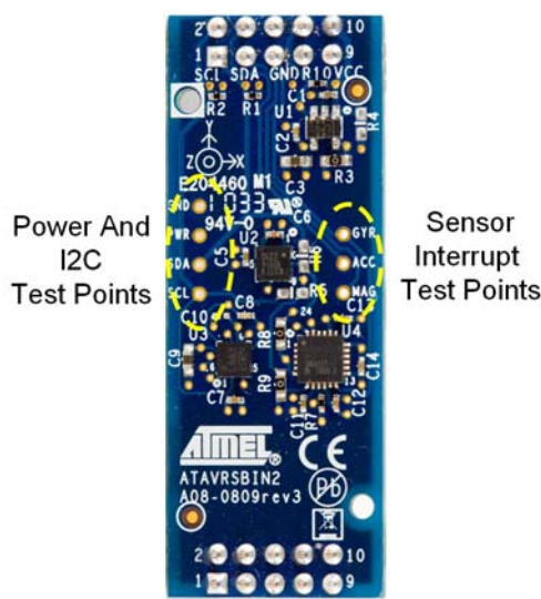
Figure 5-2. Locations of test points.
