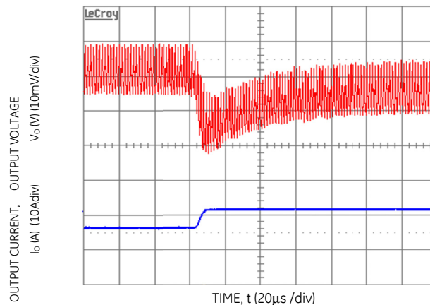
Figure 10. Transient Response to Dynamic Load Change from 50% to 100% at 12Vin, C_{out}=1\times 47\mu F+3\times 330\mu F , C_{Tune}=10nF & R_{Tune}=220ohms
