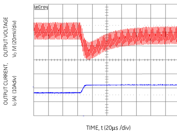
Figure 16. Transient Response to Dynamic Load Change from 50% to 100% at 12Vin, C_{out}=1\times 47\mu\text{F}+2\times 330\mu\text{F} , CTune-5600pF & RTune-270ohms
