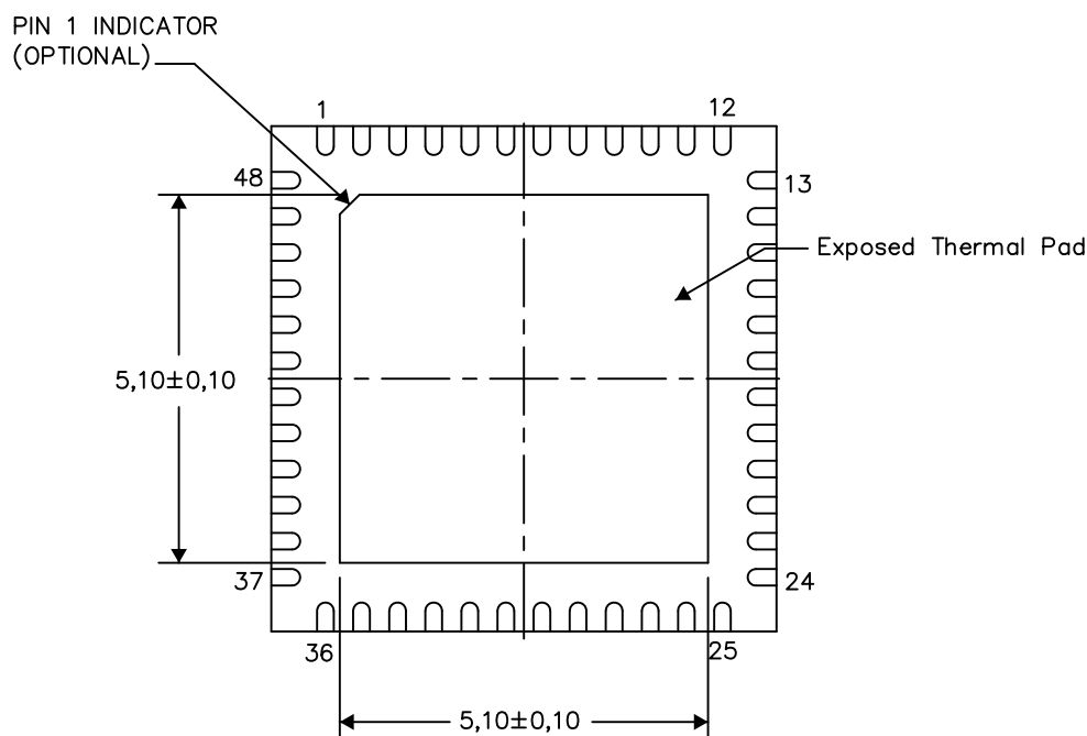
Bottom View
