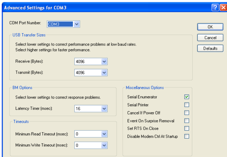
Figure 2.8 – Advanced Options
