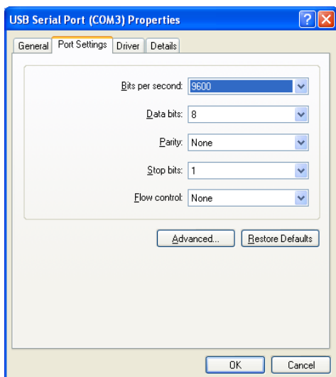
Figure 2.7 – Settings Tab
