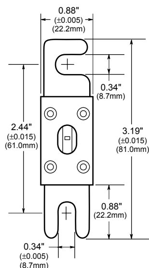
Dimensional Data
