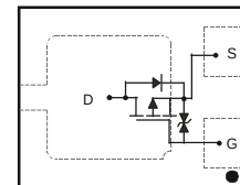
Internal Schematic
