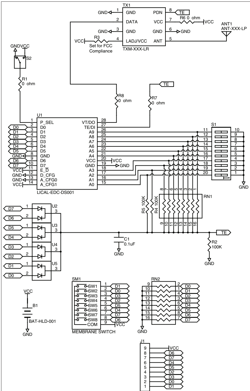
Figure 12: CMD-HHLR-***-MD Schematic
