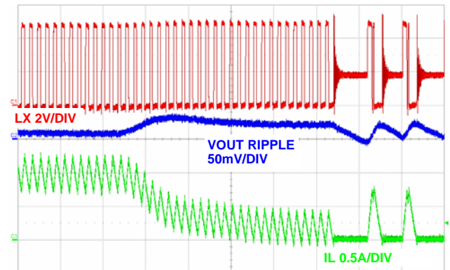
FIGURE 18. MODE TRANSITION CCM TO DCM, (5µs/DIV)
