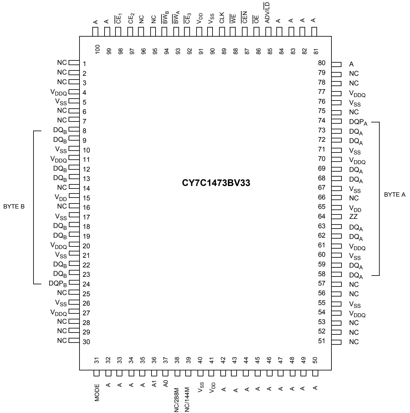
CY7C1473BV33 (4 M × 18)
