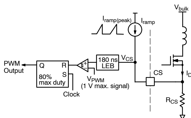
Figure 30. Current-Mode Implementation
