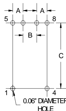
Board Layout
