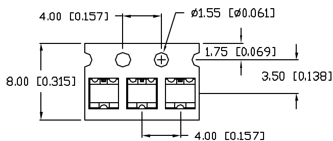
TAPE FEED DIRECTION
