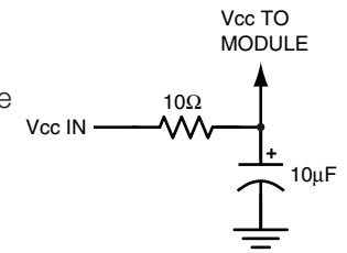
Figure 14: Supply Filter
