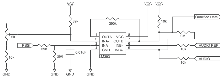
Figure 13: ES Series Receiver Squelch / Hysteresis Circuit
