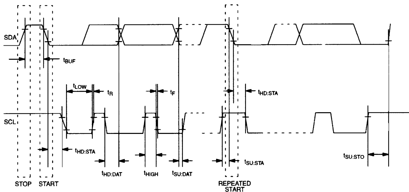
Figure 5. Timing Diagram
