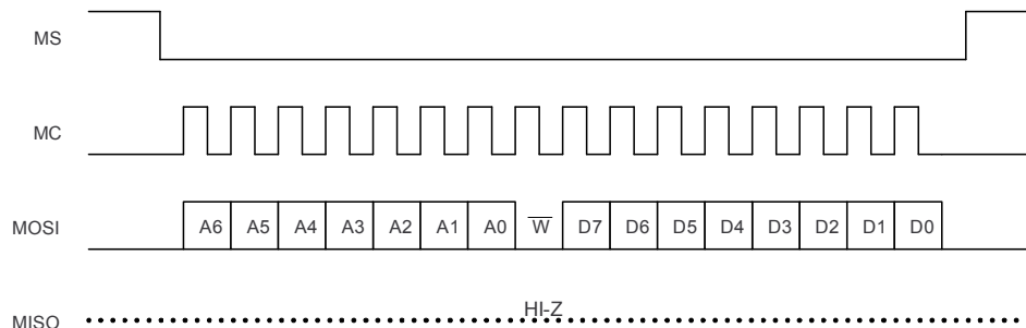
Figure 82. Serial Control Format; Write, Single Byte
