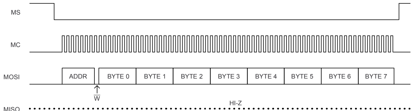
Figure 83. Serial Control Format; Write, Multiple Byte
