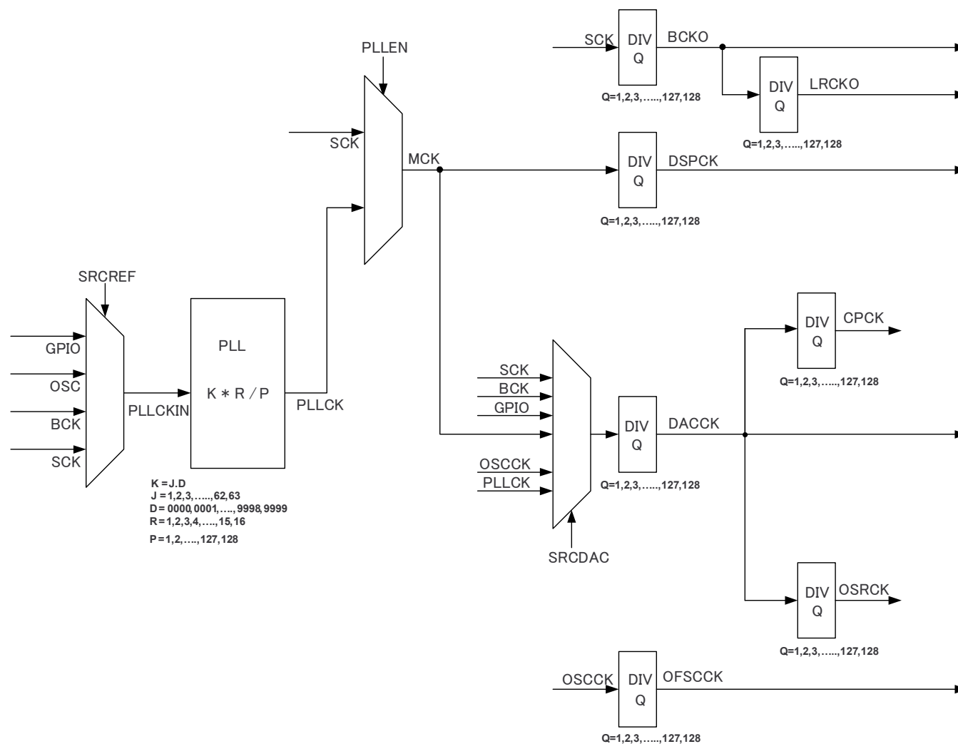
Figure 26. PLL Clock Source and Clock Distribution
