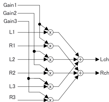
Figure 74. Figure 4. Stereo Mixer Block
