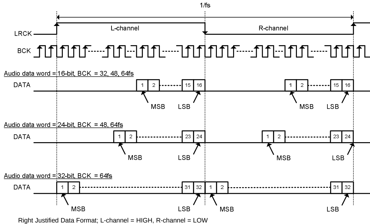
Figure 31. Right Justified Audio Data Format
