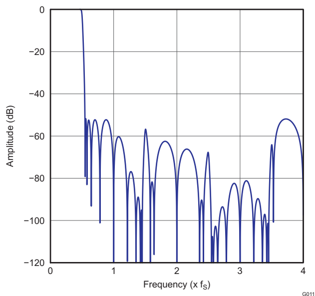
Figure 44. Low latency x8 Interpolation Filter Frequency Response
