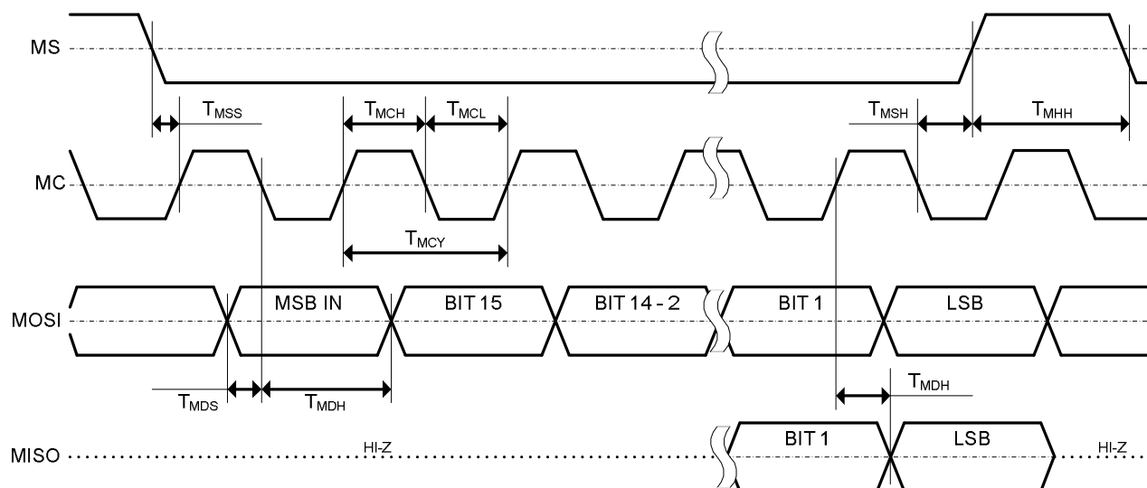
Figure 86. Control Interface Timing
