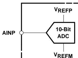
Figure 42. Single-Ended Input Stage
