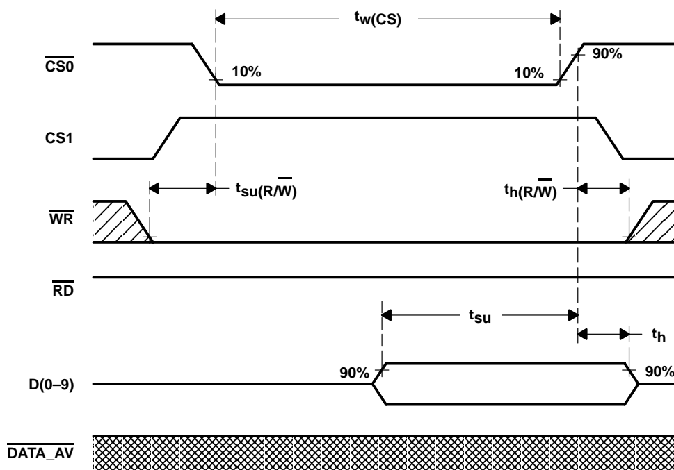
Figure 39. Write Timing Diagram Using \overline{\text{R/W}} ( \overline{\text{CS0}} -controlled)
