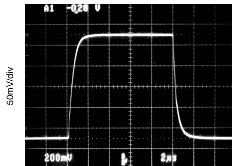
SMALL SIGNAL STEP RESPONSE G = 3 , C_L = 1000pF
