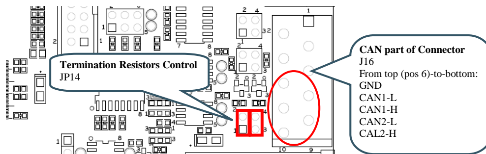
Figure 19 – CAN Interface
