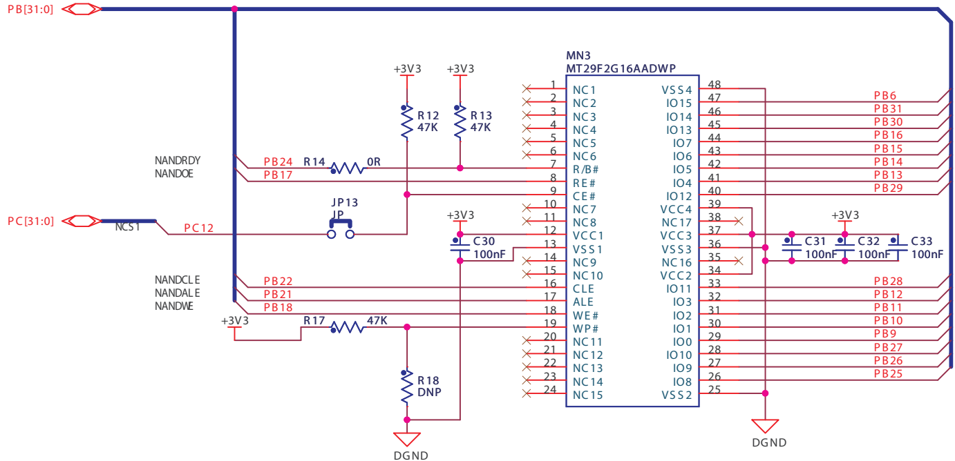
Figure 4-3. NAND Flash
