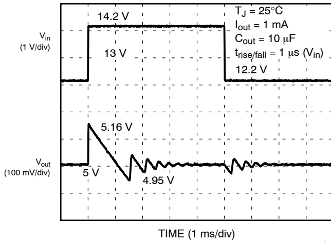
Figure 18. Line Transients (5 V Option)
