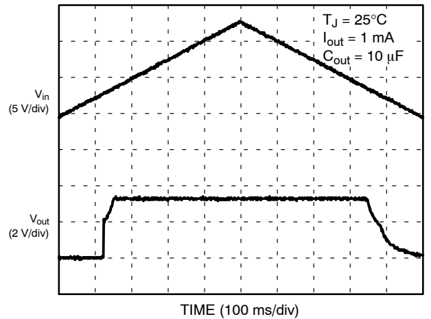
Figure 23. Power Up/Down Response (3.3 V Option)
