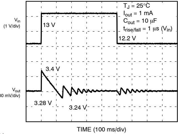
Figure 19. Line Transients (3.3 V Option)
