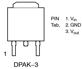
Figure 3. Pin Connections
