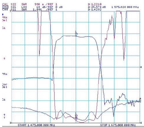
S21: LNA Gain
