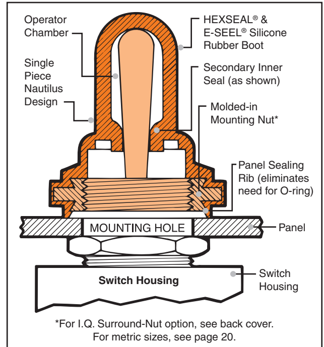
Full-Toggle Boot with Integral Secondary Inner Seal – IP66/68 Rated
