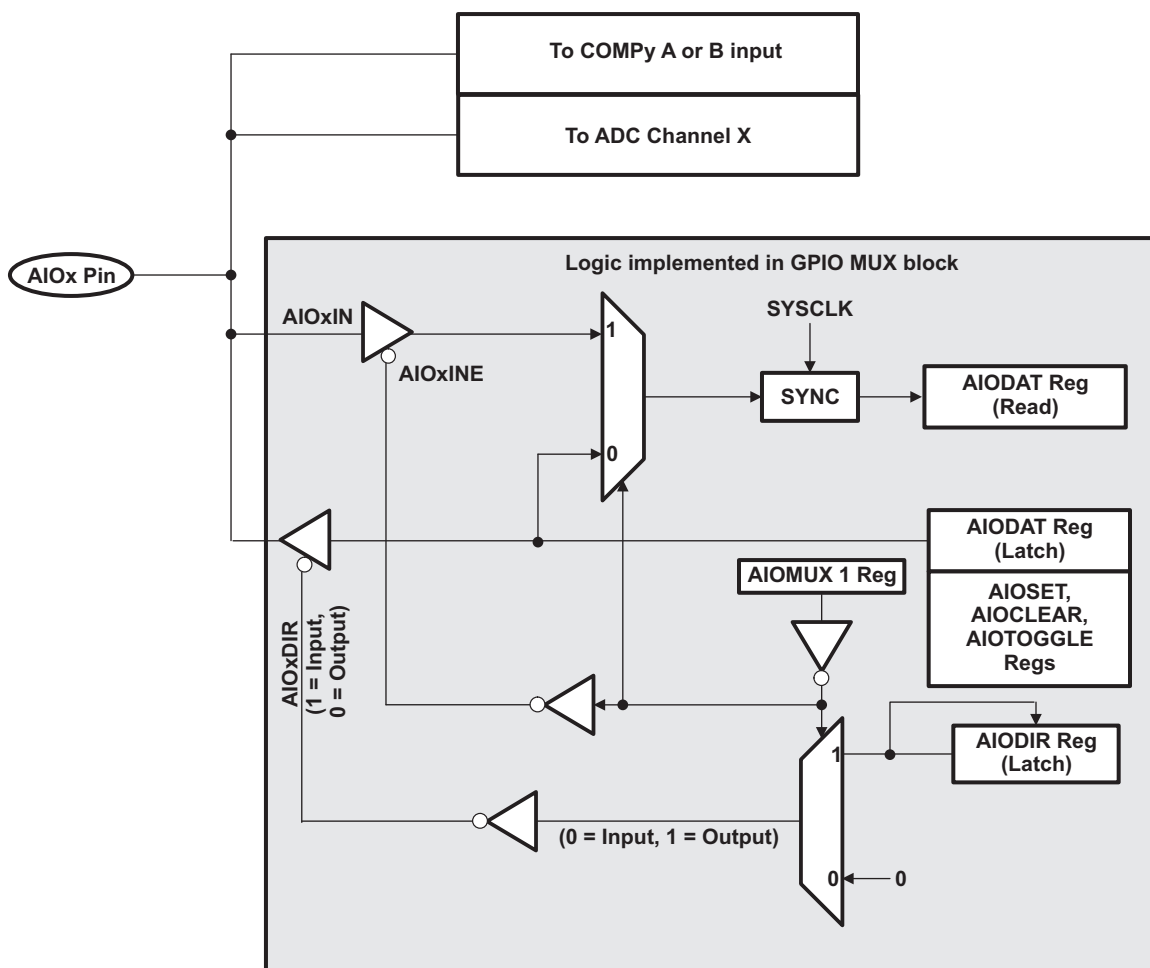
Figure 6-28. AlOx Pin Multiplexing
