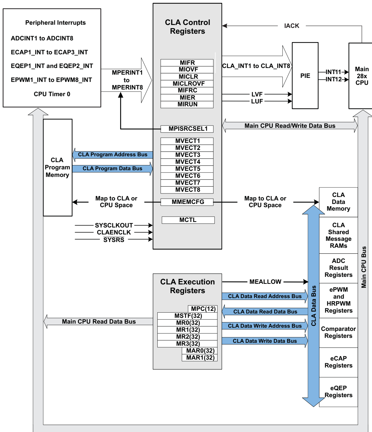
Figure 6-18. CLA Block Diagram
