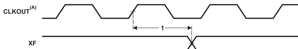
Figure 5-14. XF Timings
