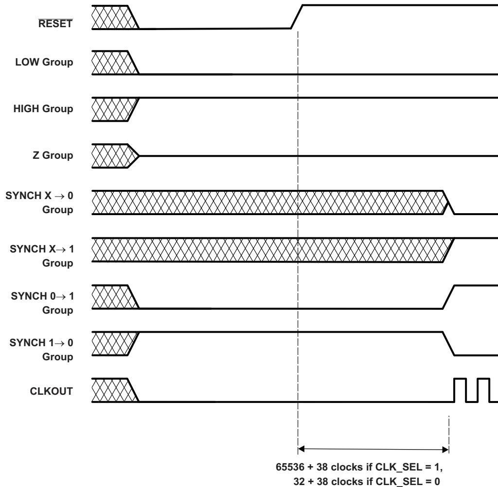
Figure 5-11. Reset Timing Requirements
