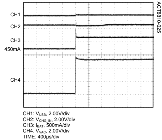
VAC Applied, CHGLEV = HIGH
