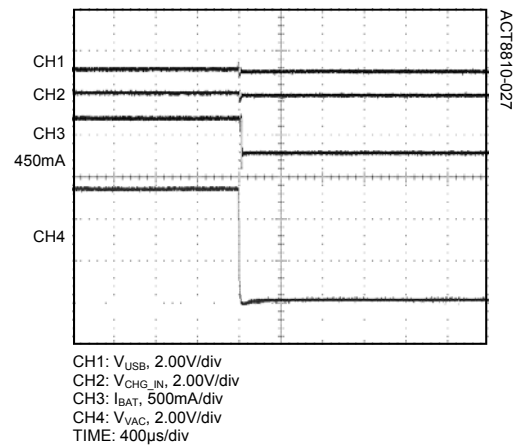
VAC Removed, CHGLEV = HIGH
