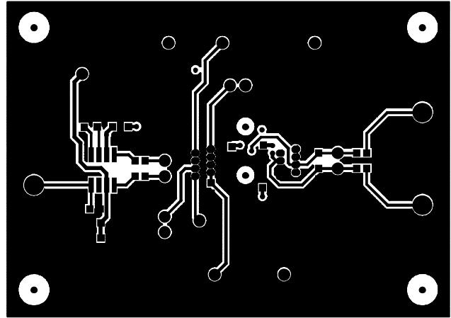
Figure 76. Wiring-Side Pattern
