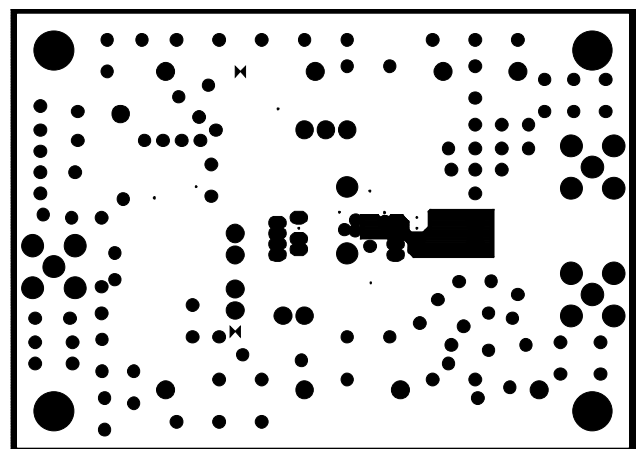
Figure 77. Inner Layer 2
