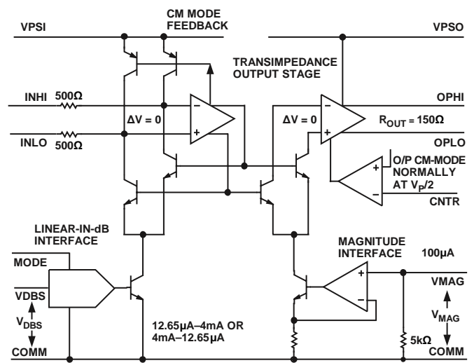
Figure 47. Schematic of Key Components
