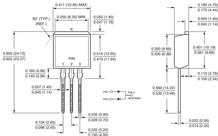
TO-262AA
