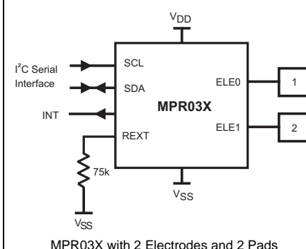
MPR03X with 2 Electrodes and 2 Pads
