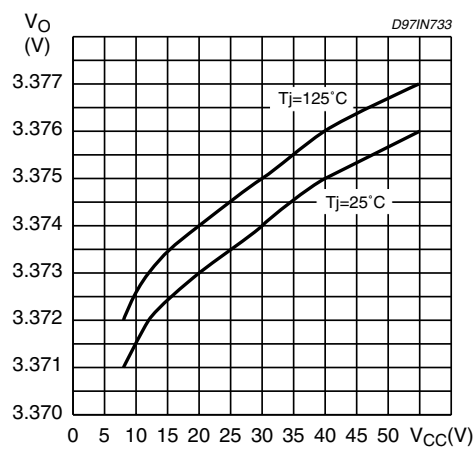
Figure 10. Load regulation
