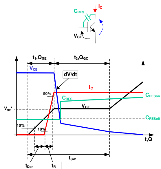
Figure 20: Nomenclature
