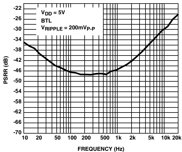
FIGURE 21. PSRR vs FREQUENCY
