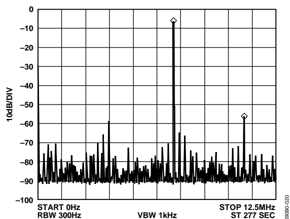
Figure 20. f_{\text{CLK}} = 25 \text{ MHz} , f_{\text{OUT}} = 7.1 \text{ MHz} , Frequency Word = 0x48B43958
