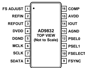
Figure 6. Pin Configuration
