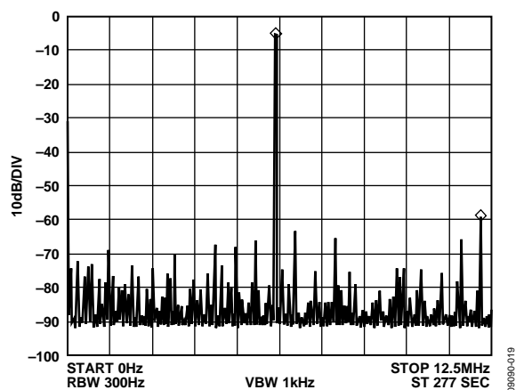
Figure 19. f_{\text{CLK}} = 25 \text{ MHz} , f_{\text{OUT}} = 6.1 \text{ MHz} , Frequency Word = 0x3E76C8B4
