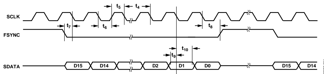
Figure 4. Serial Timing
