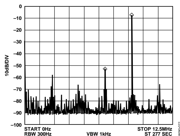
Figure 22. f_{\text{CLK}} = 25 \text{ MHz} , f_{\text{OUT}} = 9.1 \text{ MHz} , Frequency Word = 0x5D2F1AA0
