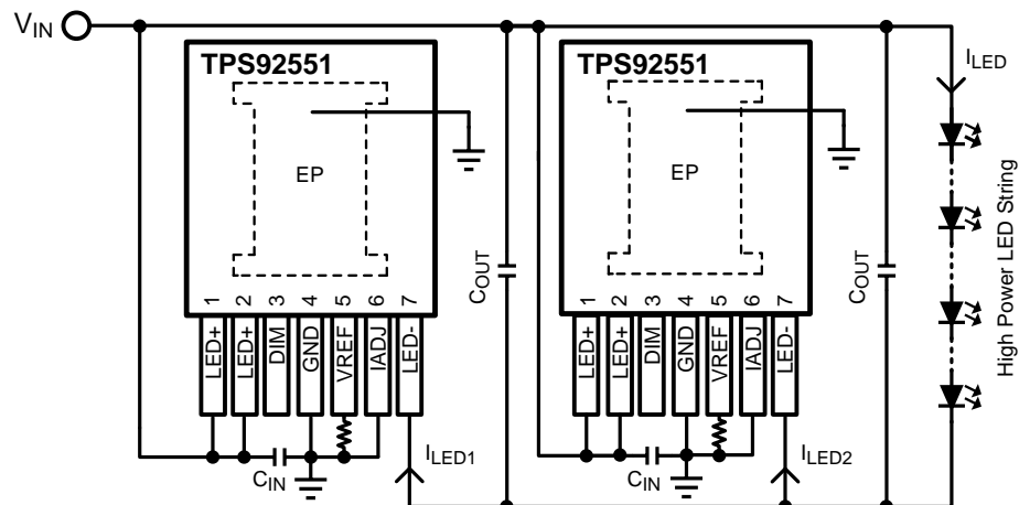
Figure 34. Parallel Operation Circuit Schematic for I_{LED} = 900\text{mA}
