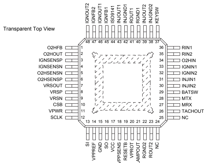
Figure 3. 33814 Pin Connections
