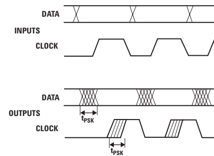
Figure 5. Parallel Data Transmission.
