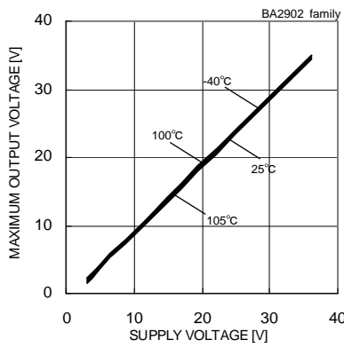
Fig. 76 Maximum Output Voltage - Supply Voltage ( R_L=10[k\Omega] )
