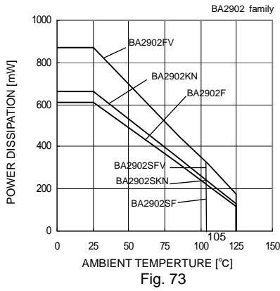
Fig. 73 Derating Curve
