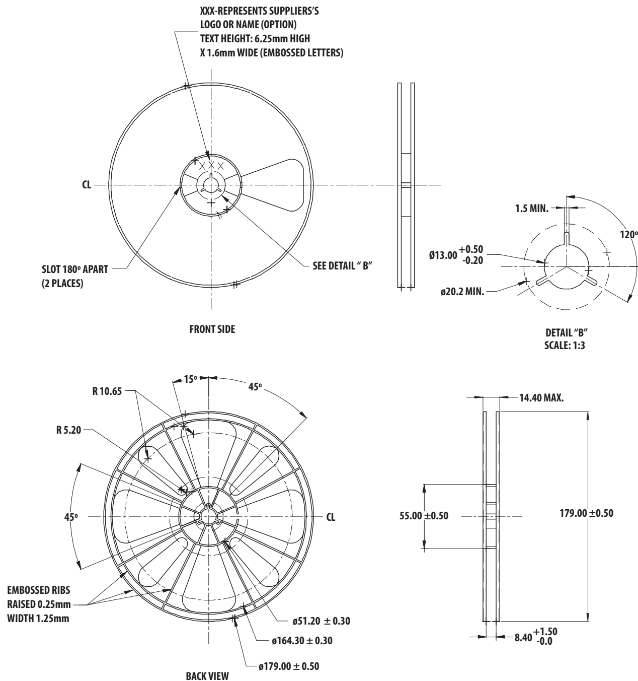
Figure 14. Reel Dimension Drawing
