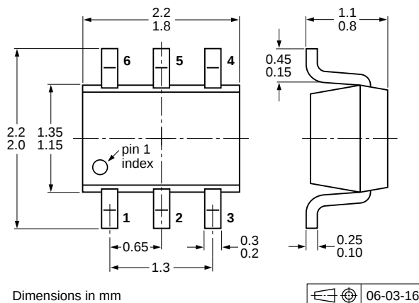
Fig 11. Package outline PUMB9 (SOT363)
