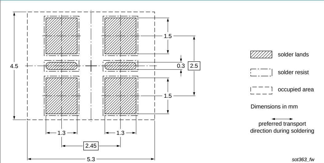
Fig 14. Wave soldering footprint PUMB9 (SOT363)
